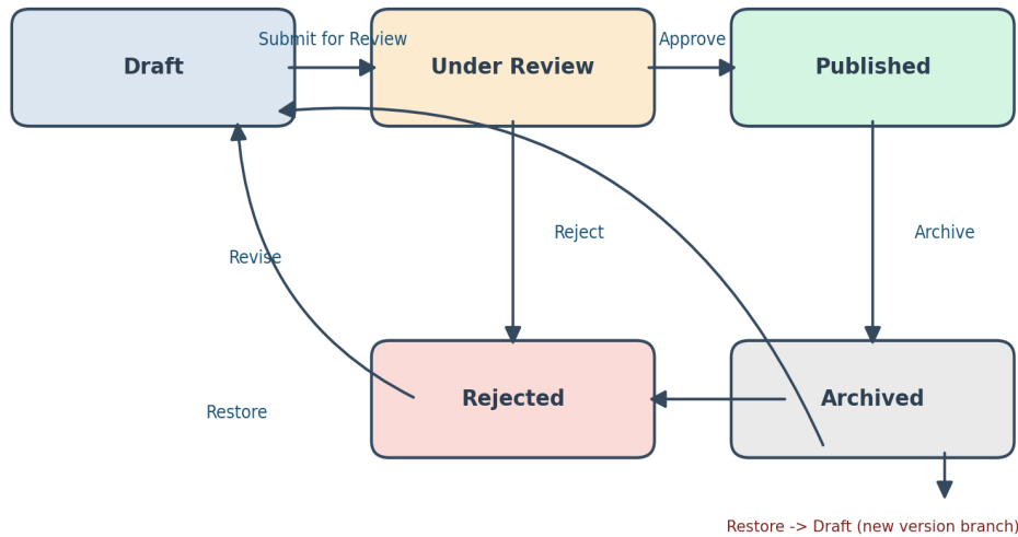
Figure 1: State Transition Diagram - Document Version Lifecycle
